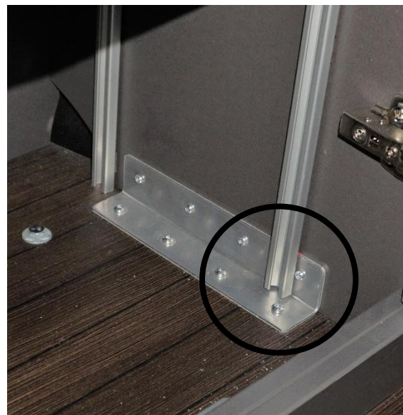
Figure 6. Positioning of aluminium track (B) right hand side.
